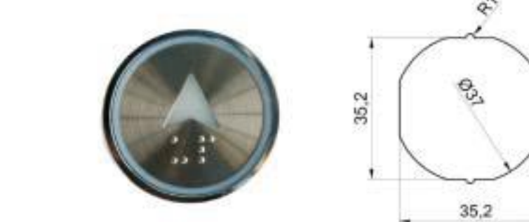
SH-EPB313B-C
