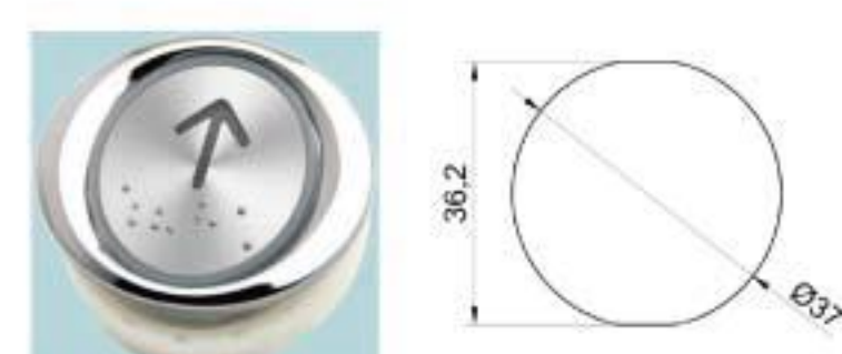
SH-EPB123
