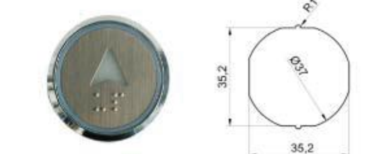
SH-EPB313B-X
