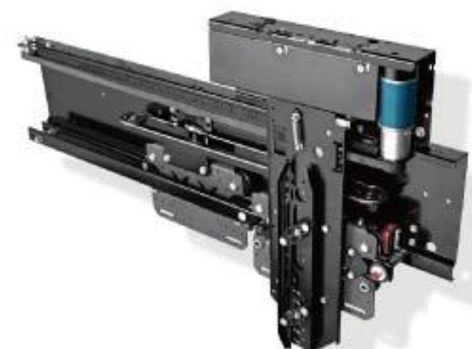
SH-ECO-12/R-L Two Panels Telescopic Opening Car Door Operator
