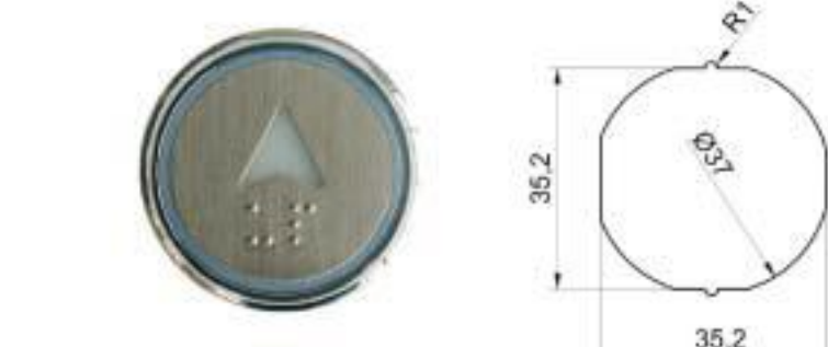
SH-EPB313-O
