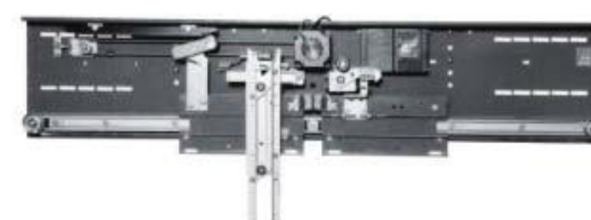
SH-131-50-YC-A
