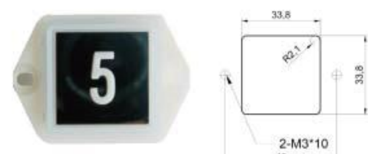
SH-EPB322-FS
