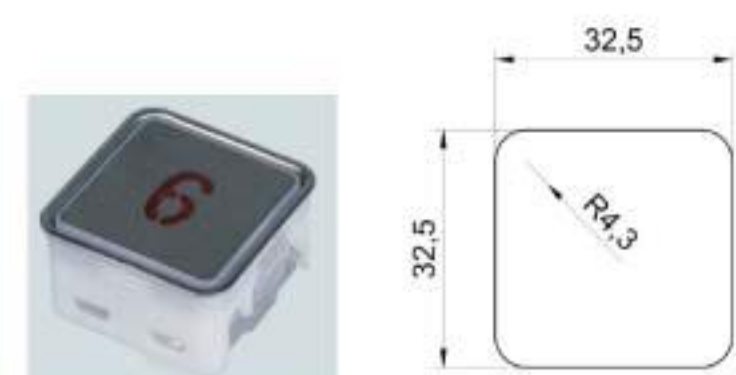
SH-EPB270
