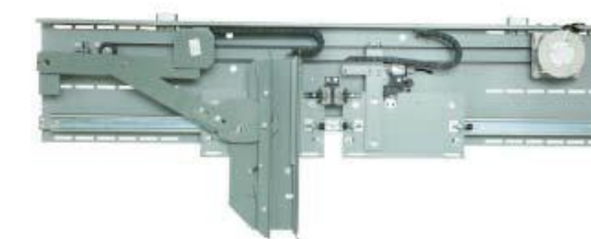
SH-MP-211 Center Opening Two Panel Operator (Car Frame Installation)
