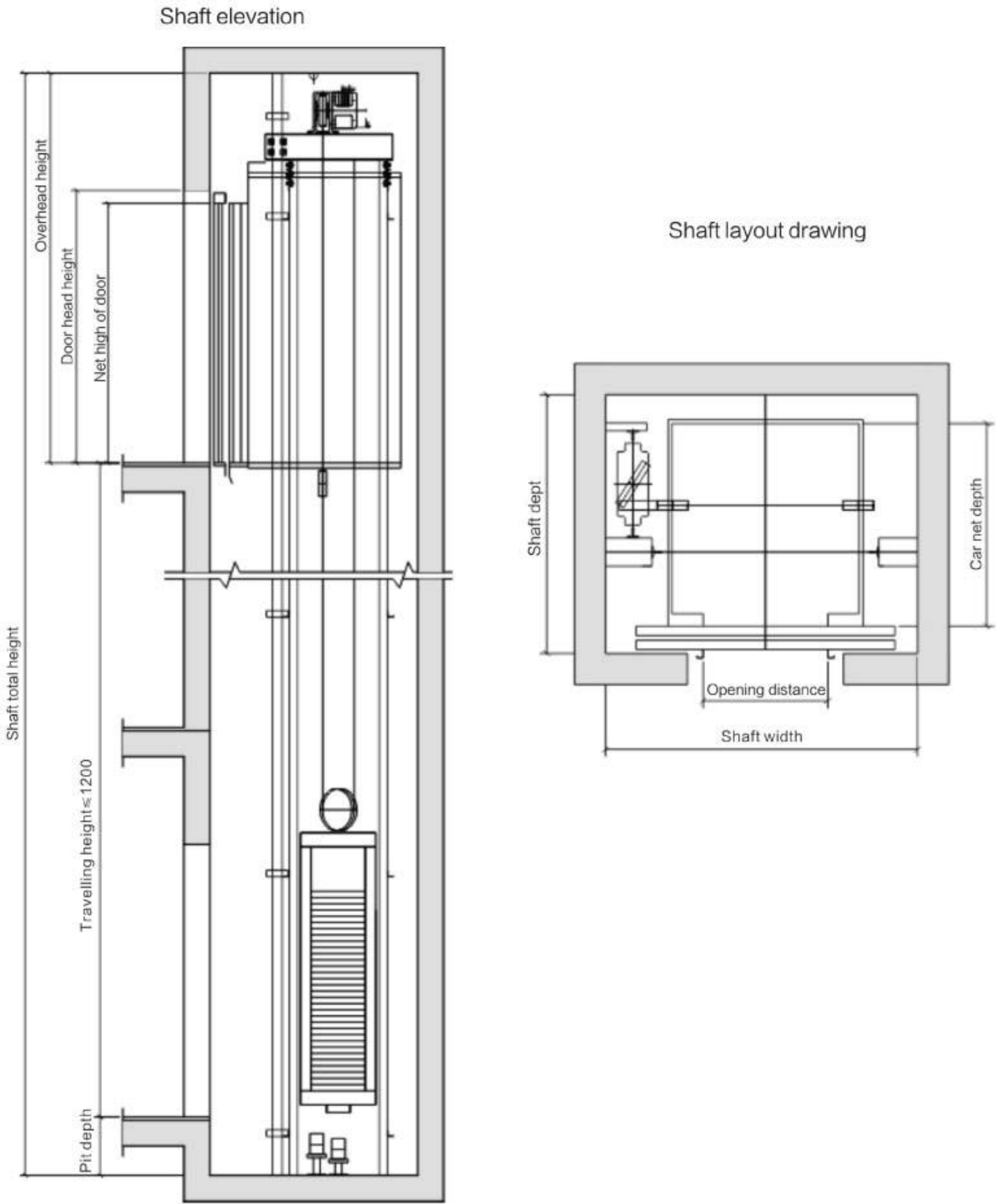
Villa elevator specifications
