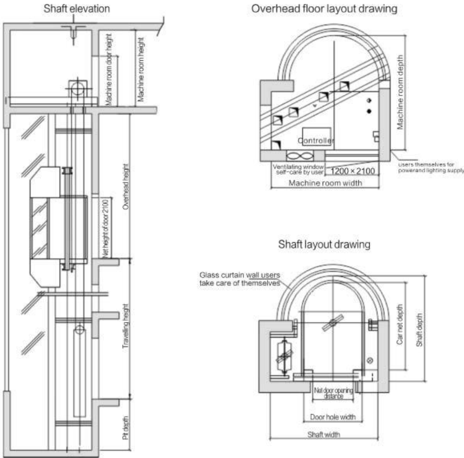
Semicircle machine room / Machine roomless elevator specifications
