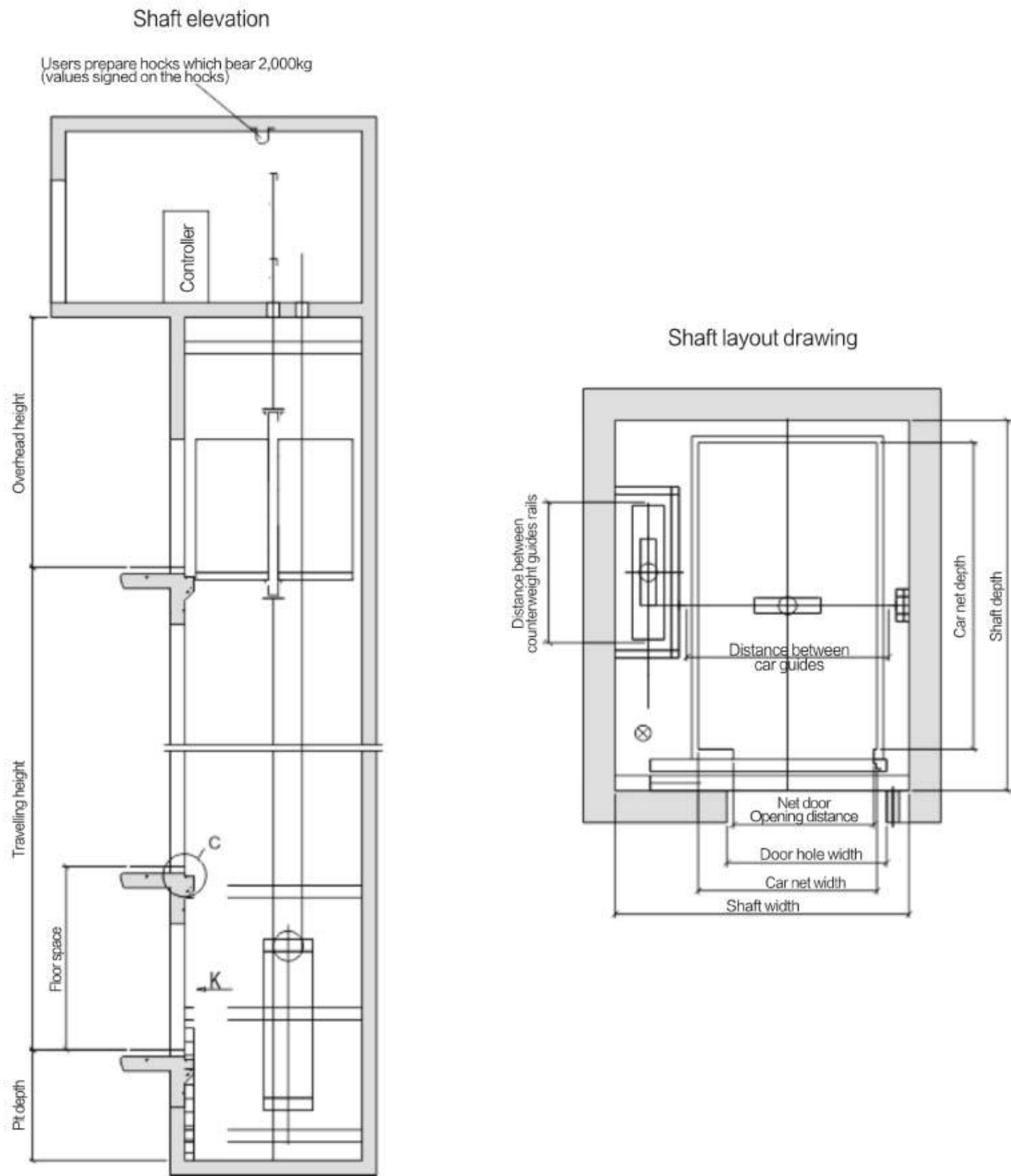
Machine room / Machine roomless bed elevator specifications
