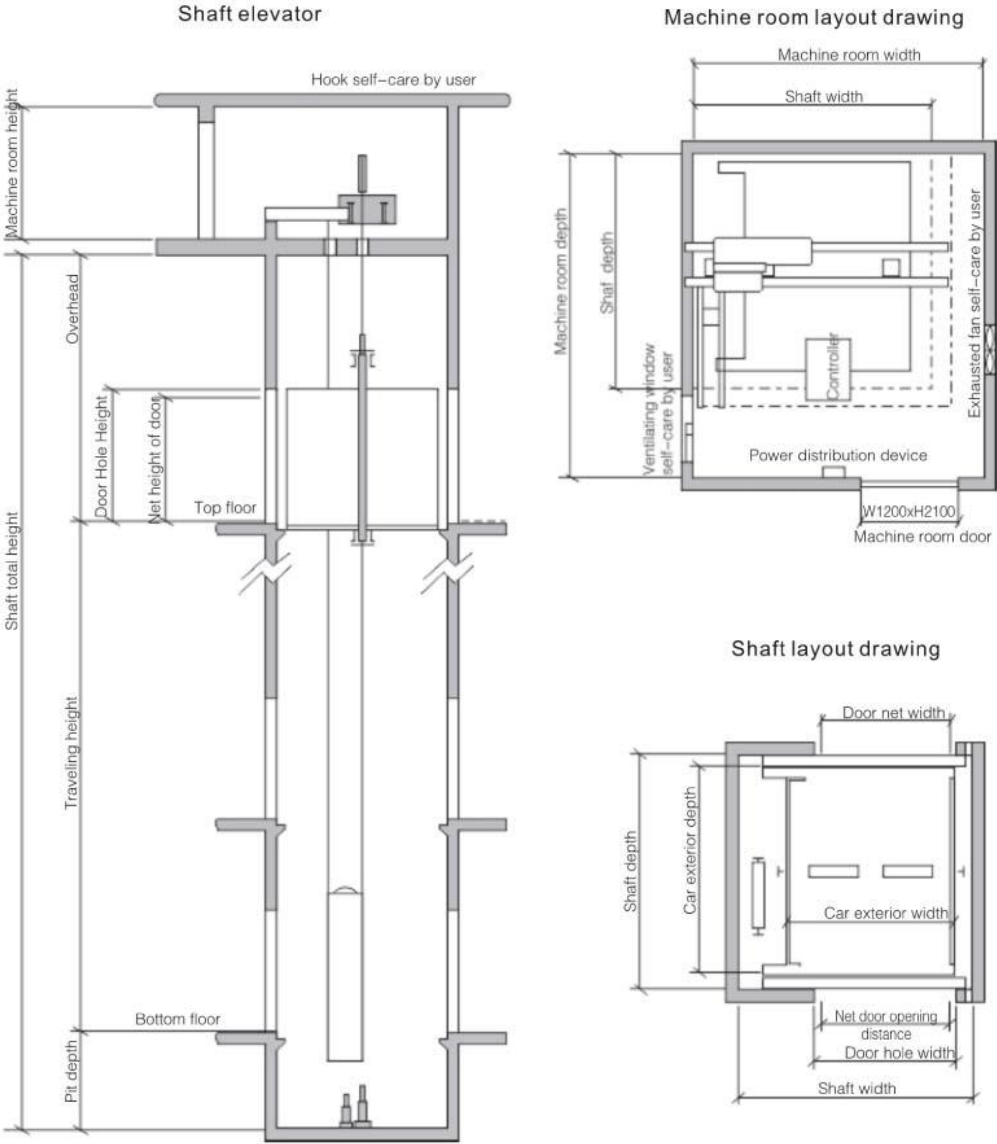
Freight elevator specifications
