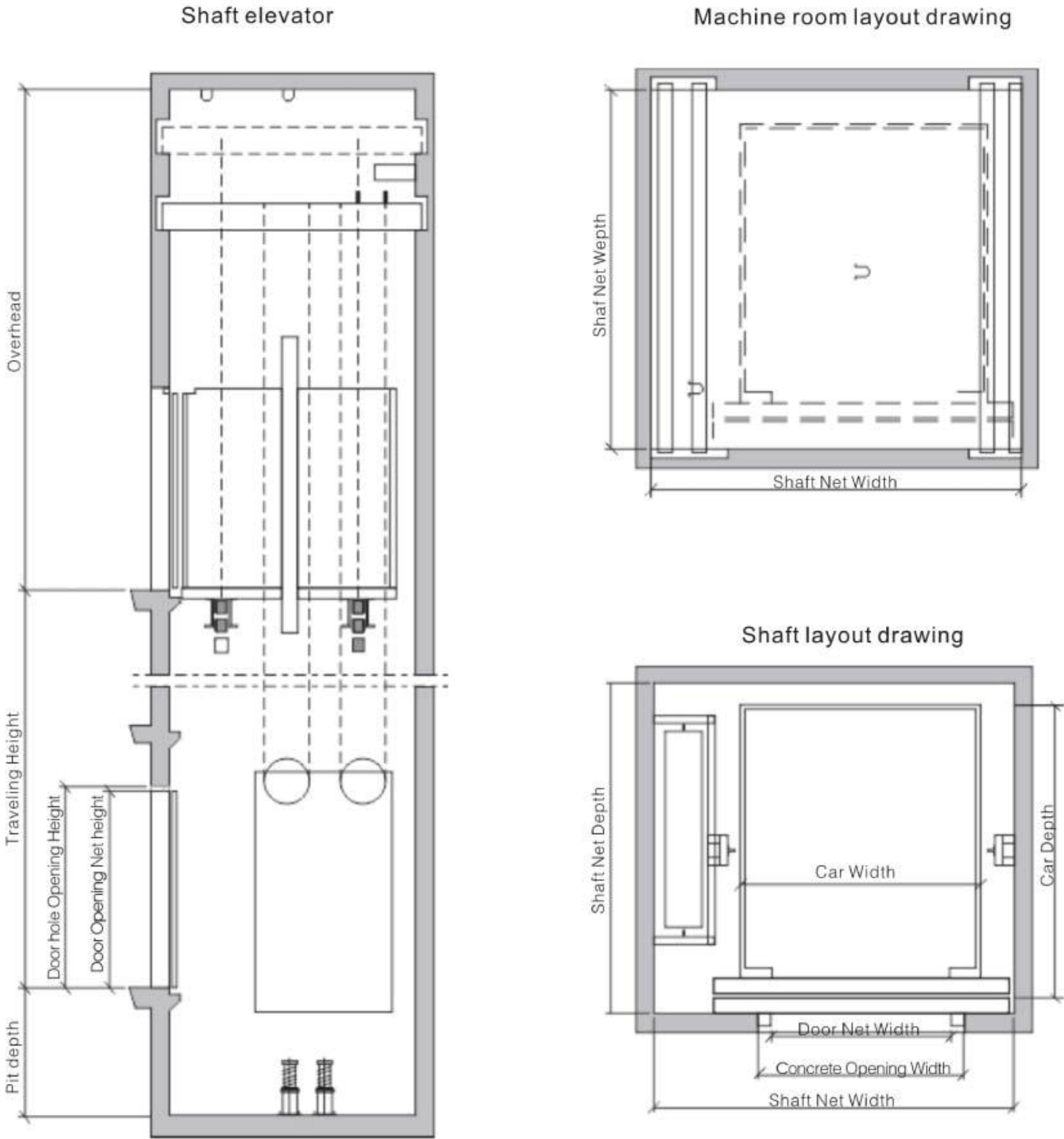
Machine roomless(MRL) freight elevator specifications
