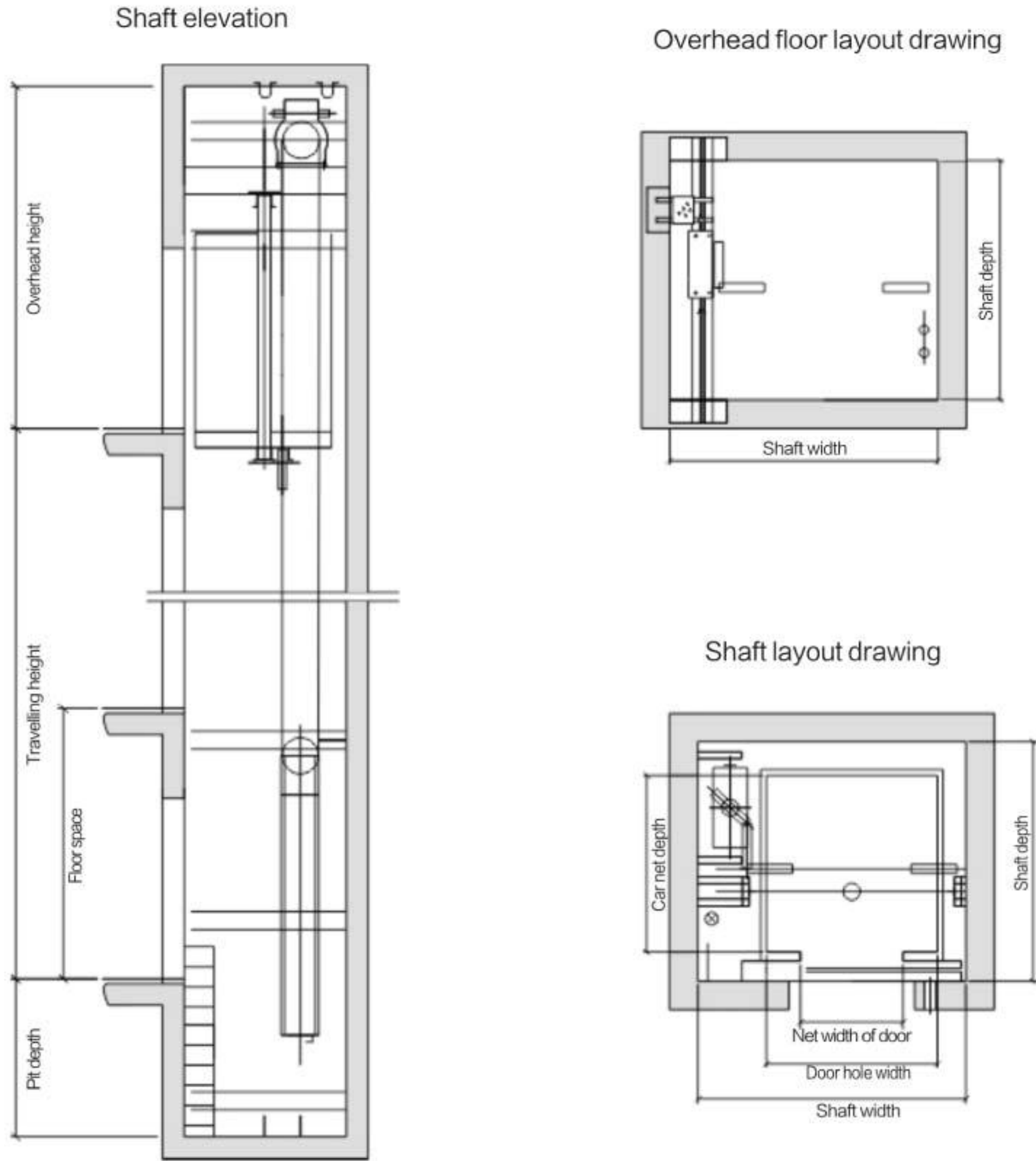
Machine roomless passenger specifications
